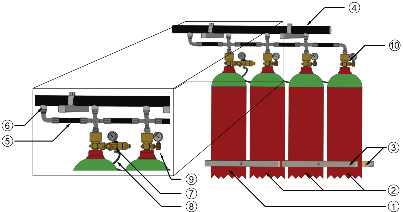
Figure 1. Single Area Container Bank Arrangement
