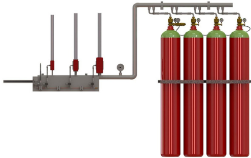
Figure 12. Selector Valve Setup
